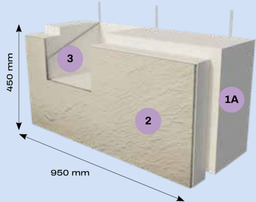
STANDARD PANEL WITH TG JOINT
