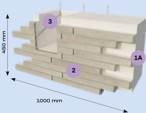
CLINKER PATTERN PANEL WITH TG JOINT
