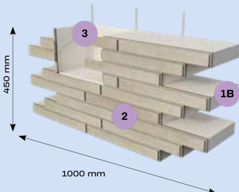
CLINKER PATTERN PANEL
